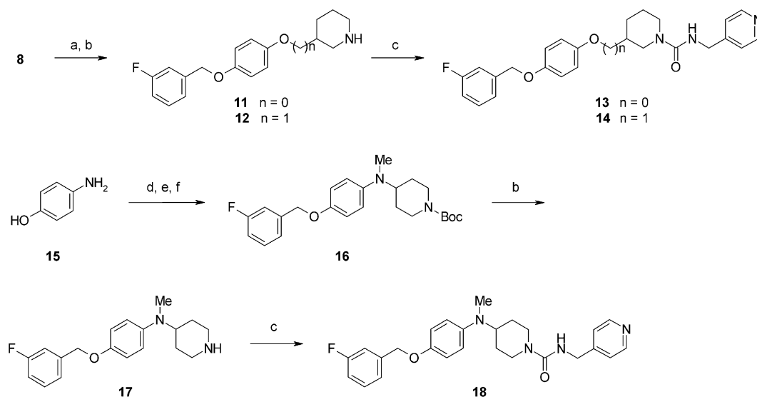
Scheme 2. Reagents and conditions: (a) DEAD, PPh 3 , t -butyl 3-hydroxypiperidine-1-carboxylate, or t -butyl 3-hydroxymethylpiperidine-1-carboxylate, THF; (b) HCl, AcOEt–MeOH; (c) bis(trichloromethyl)carbonate, Et 3 N, THF, then pyridin-4-ylmethylamine; (d) 1-(bromomethyl)-3-fluorobenzene, t -BuOK, DMF; (e) t -butyl 4-oxopiperidine-1-carboxylate, NaBH(OAc) 3 , AcOH; (f) formaldehyde, NaBH(OAc) 3 , AcOH.
