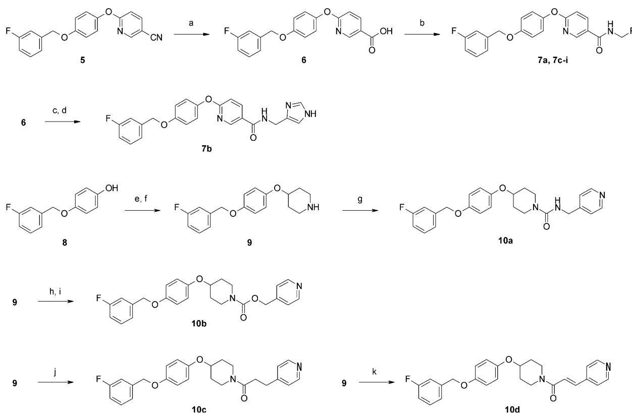
Scheme 1. Reagents and conditions: (a) 5 M NaOH, EtOH, reflux; (b) WSC·HCl, HOBT, RCH 2 NH 2 , THF; (c) WSC·HCl, HOBT, (1-trityl-1 H -imidazol-4-yl)methylamine, THF; (d) AcOH, 70 °C; (e) PPh 3 , t -butyl 4-hydroxypiperidine-1-carboxylate, DEAD, THF; (f) HCl, AcOEt–MeOH; (g) bis(trichloromethyl)carbonate, Et 3 N, THF, then pyridin-4-ylmethylamine; (h) methyl chloroformate, Et 3 N, THF; (i) pyridin-4-ylmethanol, NaH, toluene, reflux; (j) WSC·HCl, HOBT, 3-(pyridin-4-yl)propanoic acid, THF; (k) WSC·HCl, HOBT, (2 E )-3-(pyridin-4-yl)acrylic acid, THF.
